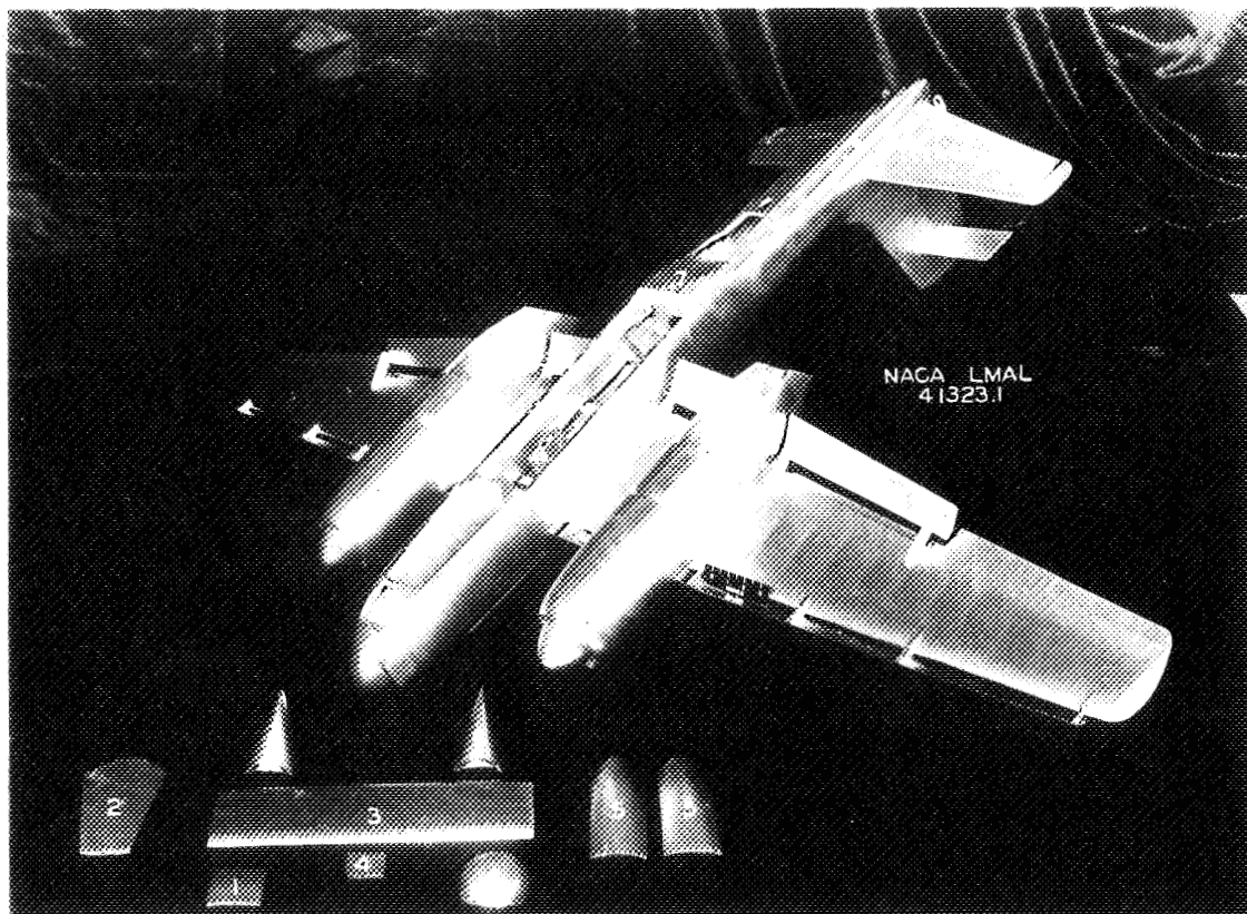
Figure 2.- Ditching model showing sections removed to simulate the various conditions of damage.
