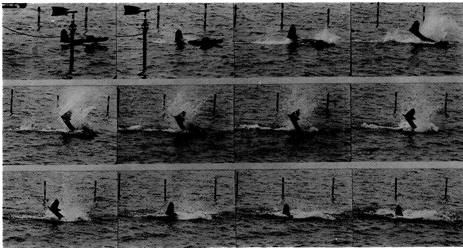
(a) Typical violent dive; ground speed, 78 mph; oncoming waves 2 feet high.
