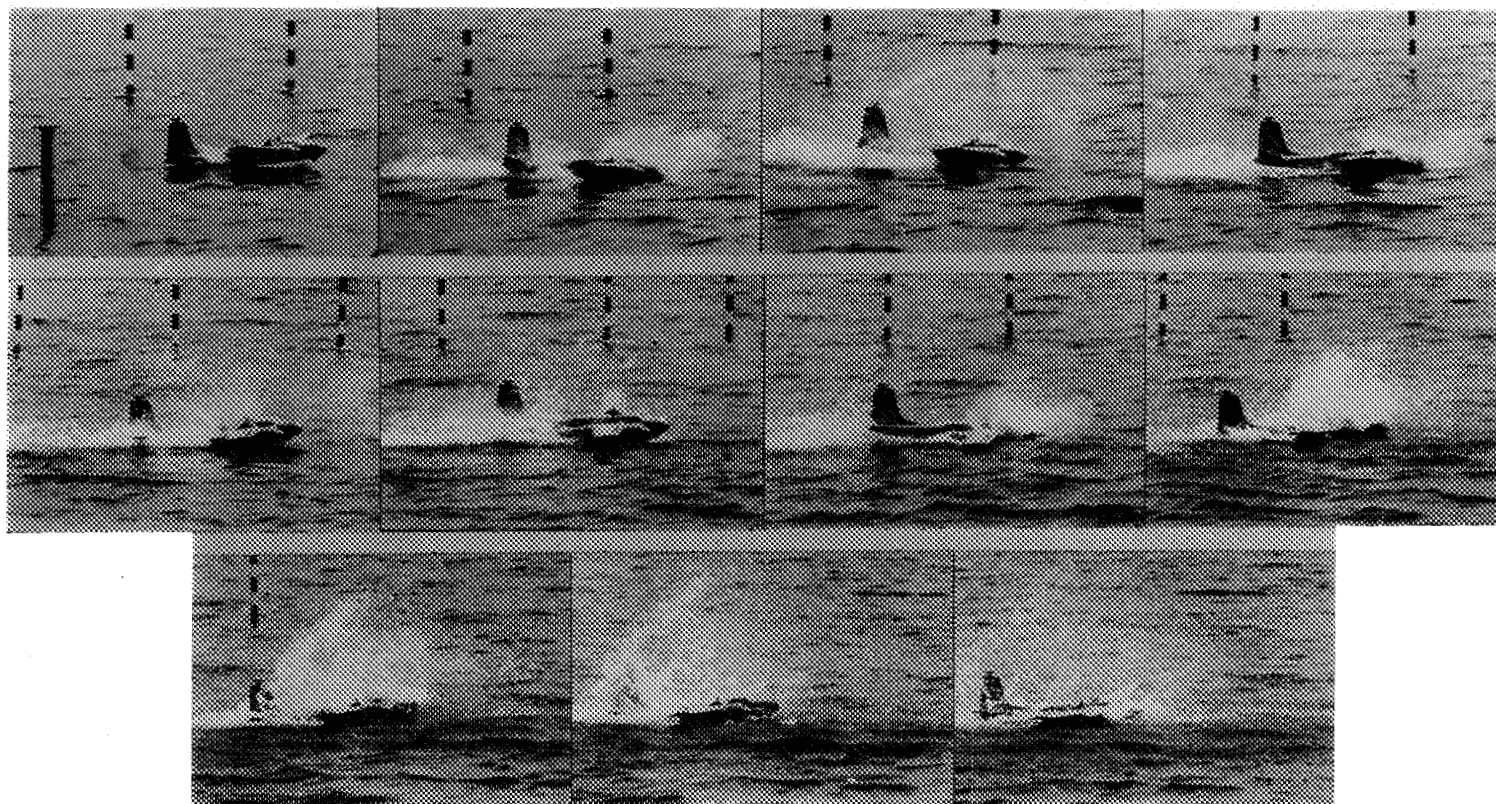
(b) Typical porpoising run obtained with hydroflap; ground speed, 100 mph; calm water.
