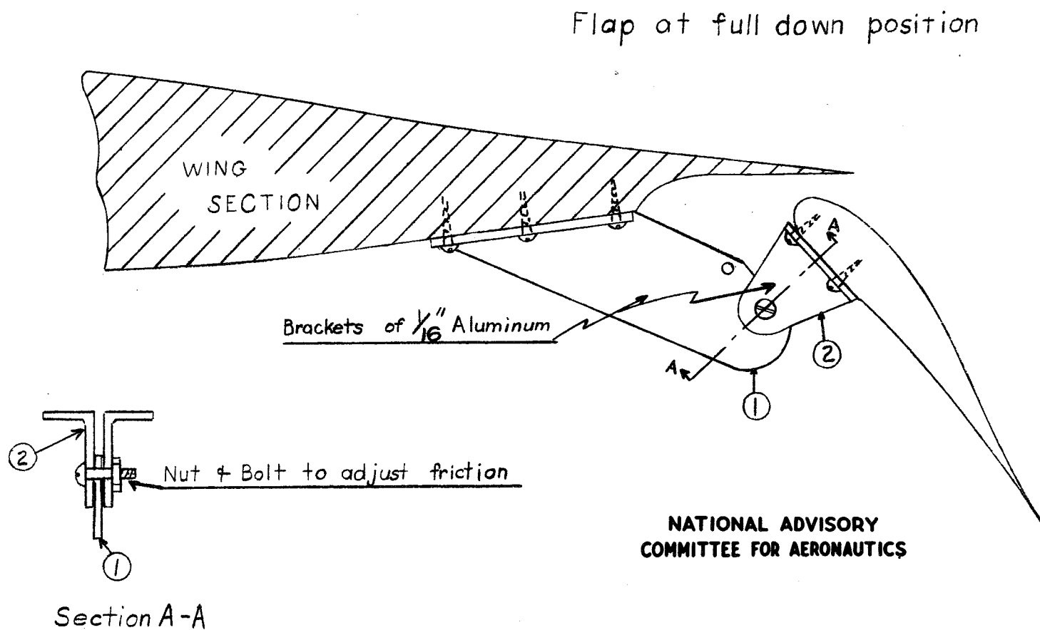
Figure 4.- Friction hinge for scale-strength flaps
