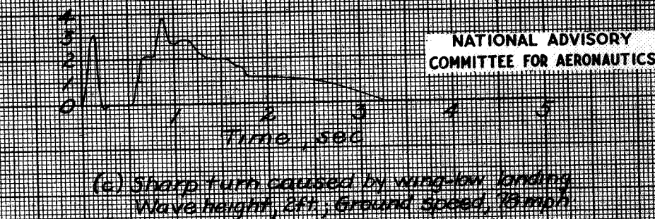
Figure 6. Typical time-histories of longitudinal decelerations for ditching tests of a 1/12 scale model of an Army P-26 airplane. Gross weight, 25,730 lb; Landing attitude 6°; Flap deflection, 35°. (All values are full-scale.)
