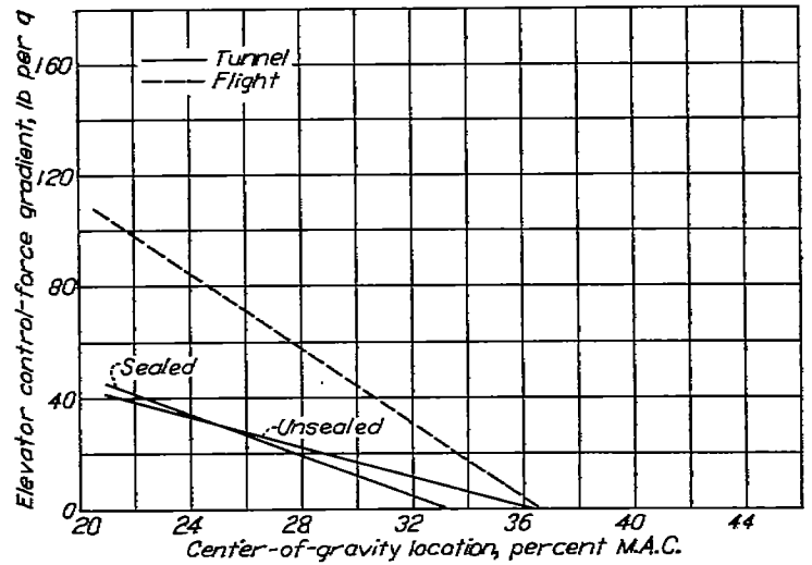
FIGURE 13.—Variation of elevator control-force gradient with center-of-gravity location estimated for sealed and unsealed elevators. V_T=280 miles per hour at 10,000-foot altitude; \delta_T=0^\circ ; rated power; steady turning flight.
