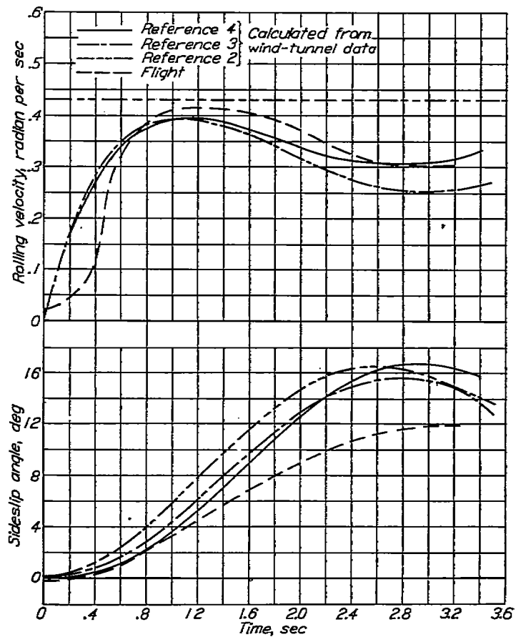
FIGURE 17.—Rolling velocity and sideslip angle during aileron roll out of 30^\circ banked turn. \delta_r = 0^\circ ; V_i = 145 miles per hour at 10,000-foot altitude; level-flight power.
