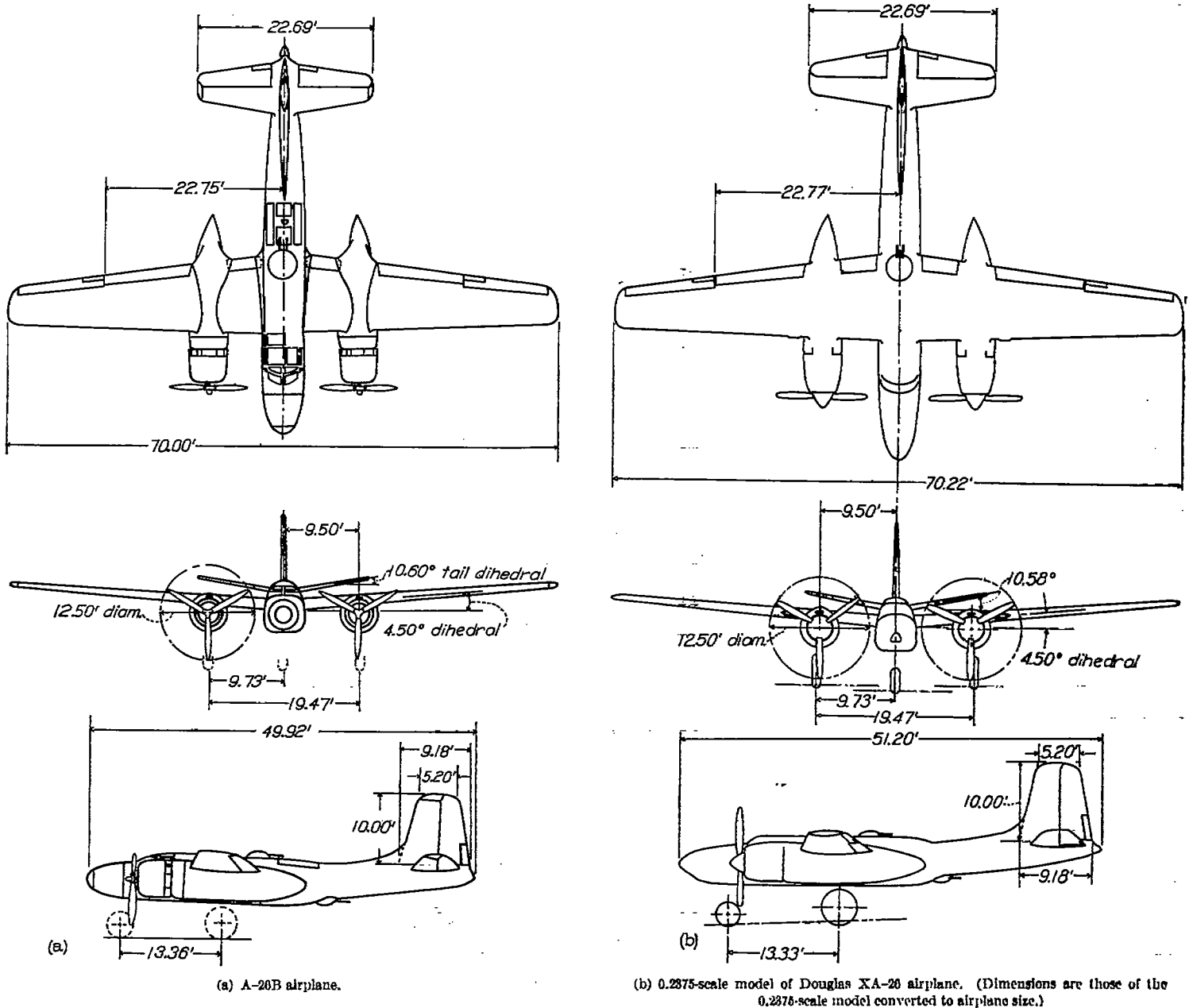
FIGURE 2.—Three-view drawings of a Douglas A-26 airplane and model.
