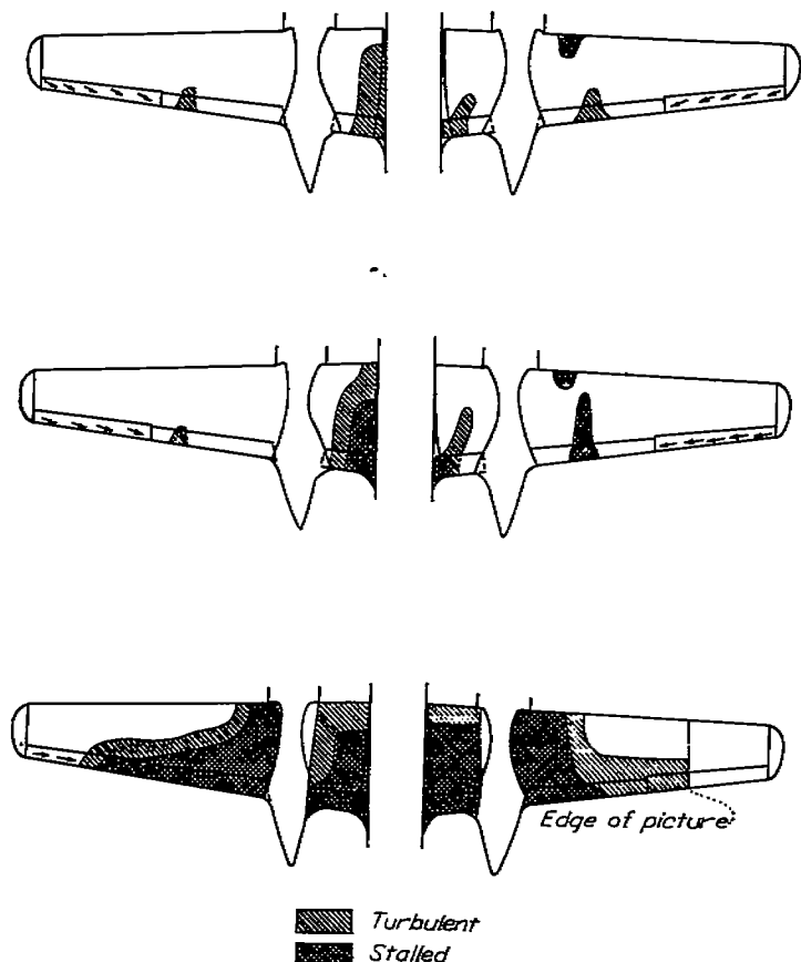
FIGURE 8.—Diagrams of stall progression in the gliding condition. Engines idling; flaps and landing gear up; cowl flaps closed; oil cooler one-half open; Douglas A-26B airplane.
