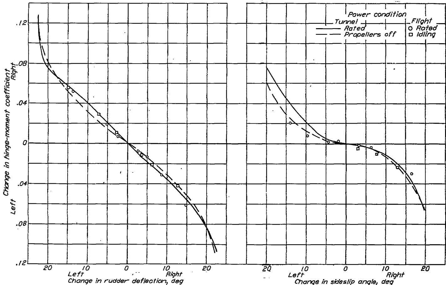
FIGURE 15.—Variation of rudder hinge-moment coefficient with rudder deflection and angle of sideslip at V=140 miles per hour. Flaps retracted.
