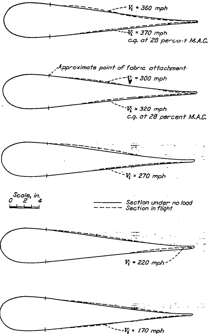
FIGURE 12.—Elevator-fabric distortion at various indicated airspeeds. No-load fabric tension, 2.7 pounds. Douglas A-26B airplane with center of gravity at 32 percent M.A.C., except where noted. Elevator section 84.2 inches from center line of airplane.
