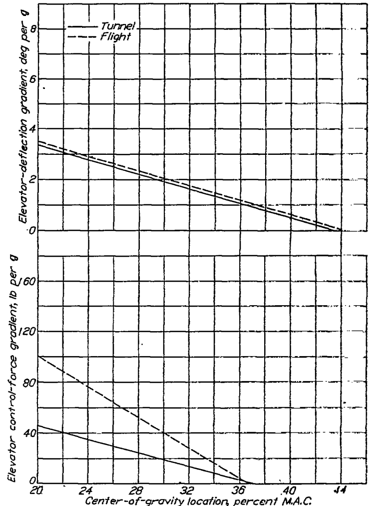
FIGURE 7.—Variation of elevator control-force and deflection gradients with center-of-gravity location. V_i=280 miles per hour at 10,000-foot altitude; \delta_s=0^\circ ; rated power; steady turning flight.
