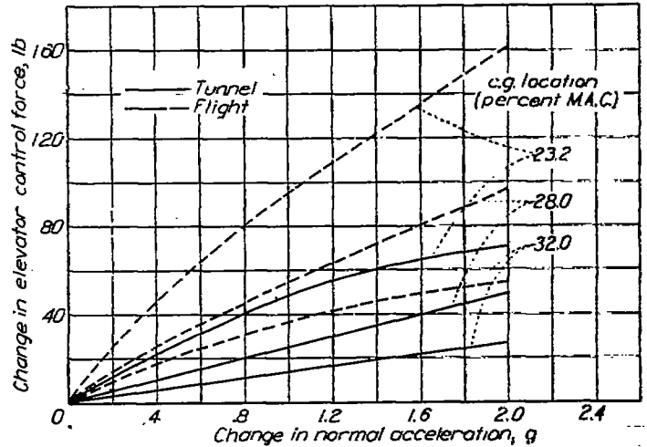
FIGURE 6.—Variation of elevator control force with normal acceleration in steady turns. V_i=280 miles per hour at 10,000-foot altitude; \delta_s=0^\circ ; rated power.
