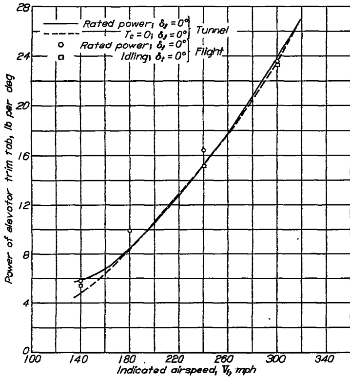
FIGURE 4.—Variation of elevator trim-tab effectiveness with airspeed.
