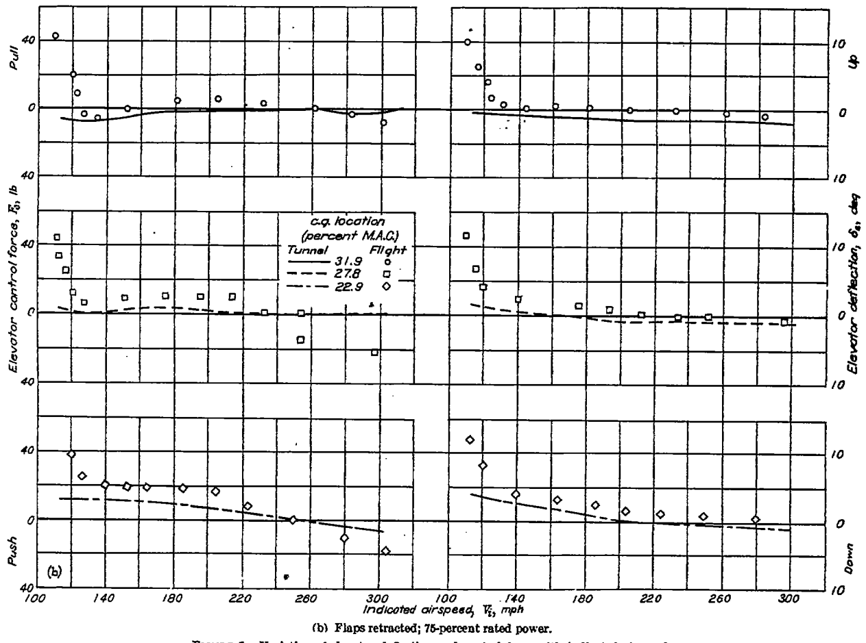
FIGURE 3.—Variation of elevator deflection and control force with indicated airspeed.
