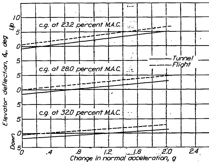
FIGURE 5.—Variation of elevator deflection with normal acceleration in steady turns. V_i=280 miles per hour at 10,000-foot altitude; \delta_s=0^\circ ; rated power.
