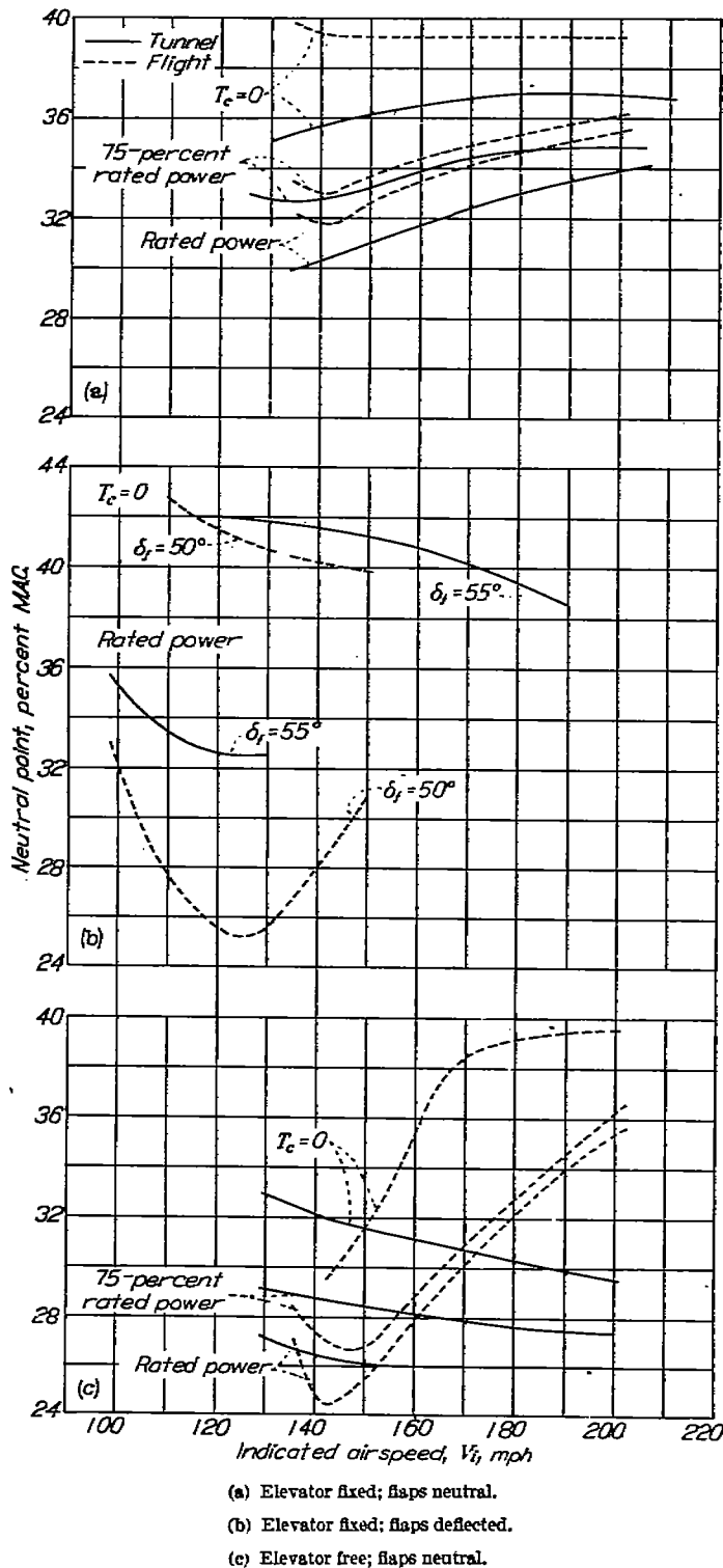
FIGURE 10.—Variation of neutral point with airspeed in straight flight.
