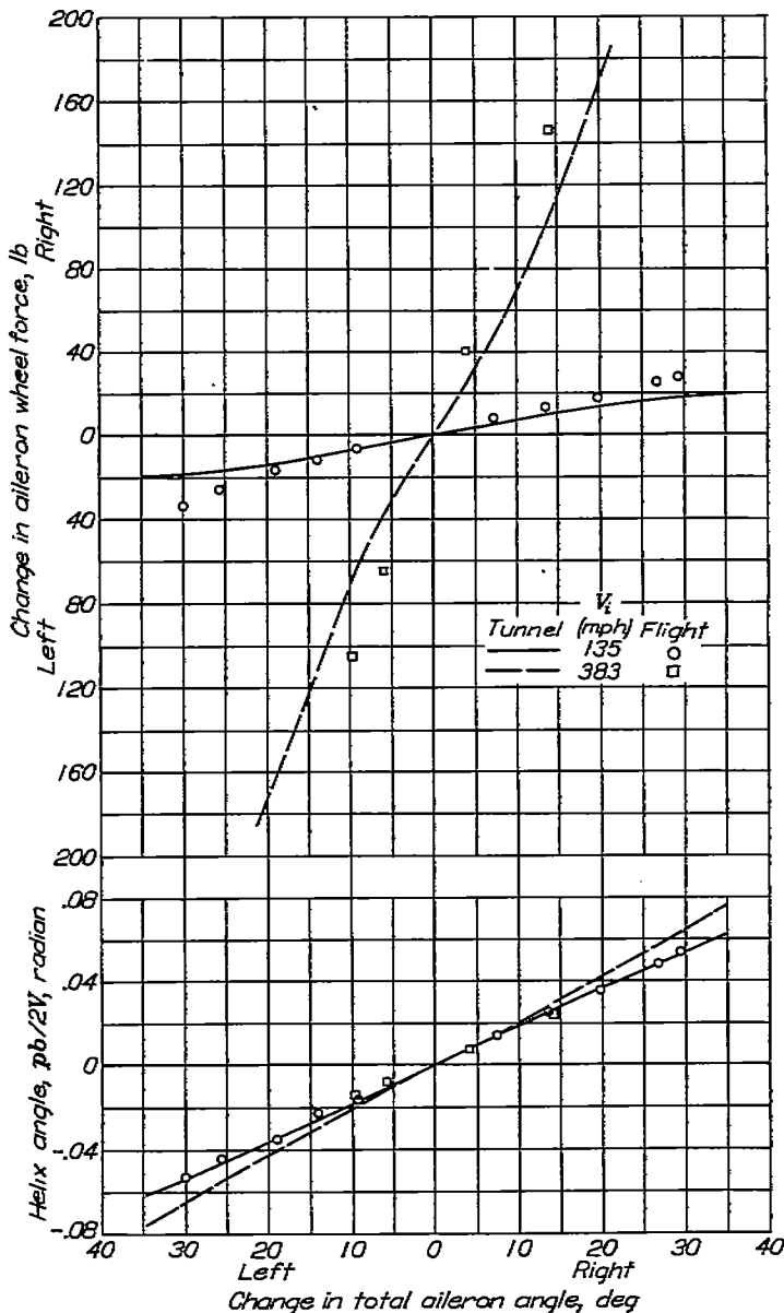
FIGURE 16.—Variation of aileron wheel force and helix angle pb/2V with change in total aileron angle in rolls with rudder fixed, flaps retracted, and rated power.
