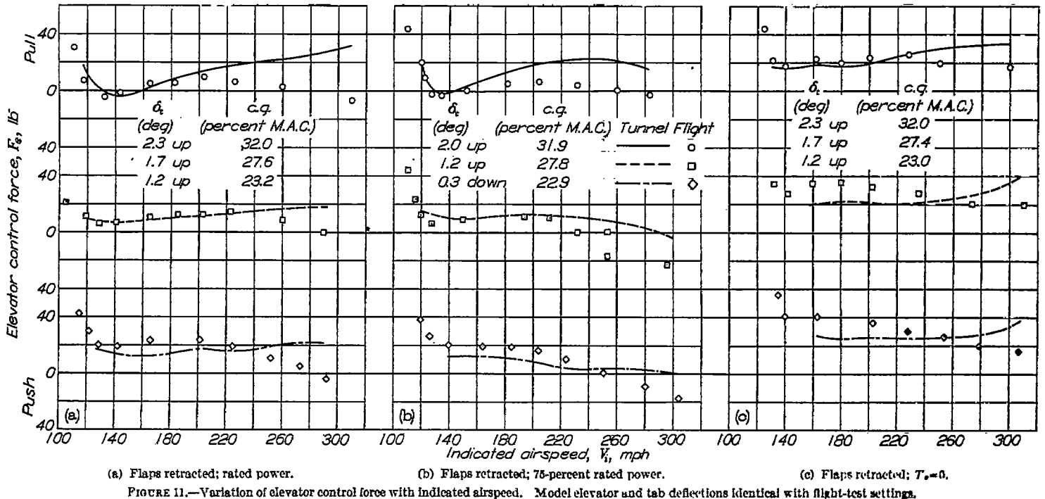
FIGURE 11.—Variation of elevator control force with indicated airspeed. Model elevator and tab deflections identical with flight-test settings.
